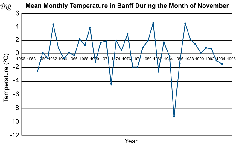
Environment Canada: Climate Change Data
